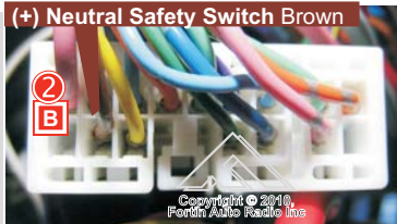
(+) Neutral Safety Switch Brown
