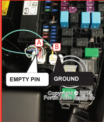
④ Engine compartment - without OEM ALARM Compartment moteur - SANS ALARME D'ORIGINE
