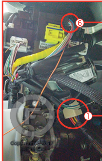
① ⑥ Steering column Colonne de direction
