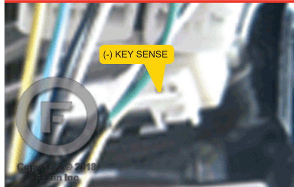
Steering column Colonne de direction
