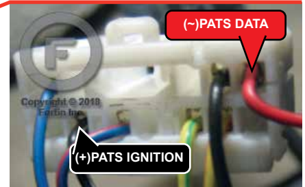
③ At Module near to the steering column Au Module proche de la colonne de direction
