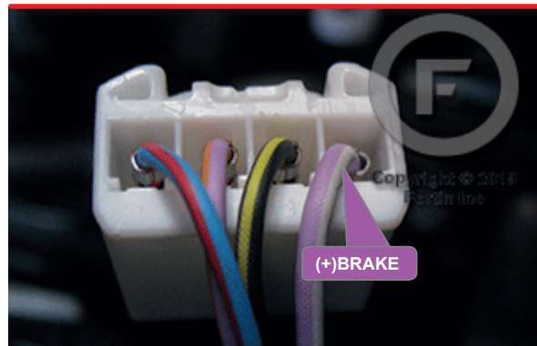
③ Foot Brake Frein
