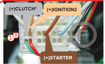
* (+)CLUTCH : Manual transmission Transmission manuelle
